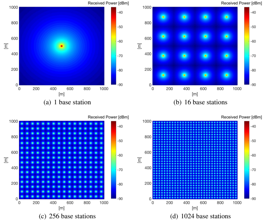
Fig. 1 Power radiated over the territory for different number of base stations - in dBm scale. A minimum power level of -90 [dBm] is ensured. The close-in propagation model of [14] with a 5G base station frequency of 3700 [MHz] is adopted. The power radiated by each base station is reduced when the number of base stations is increased (Figures best viewed in colors).
